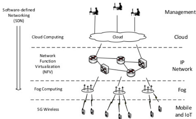
Fig. 2. Luan et al. Architecture [16].
