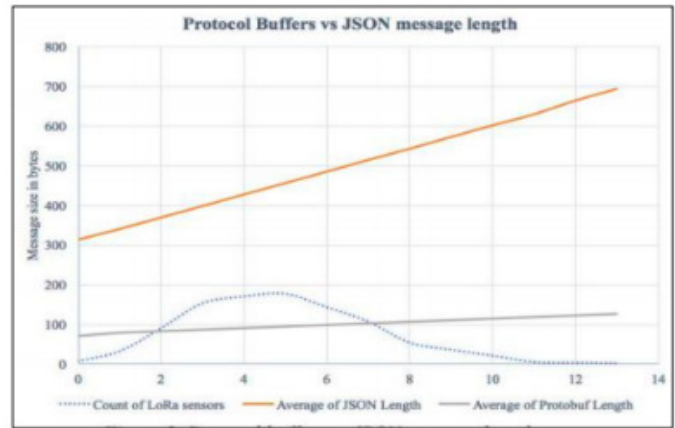
Fig. 3. Lysogor et al. performance chart [17].
